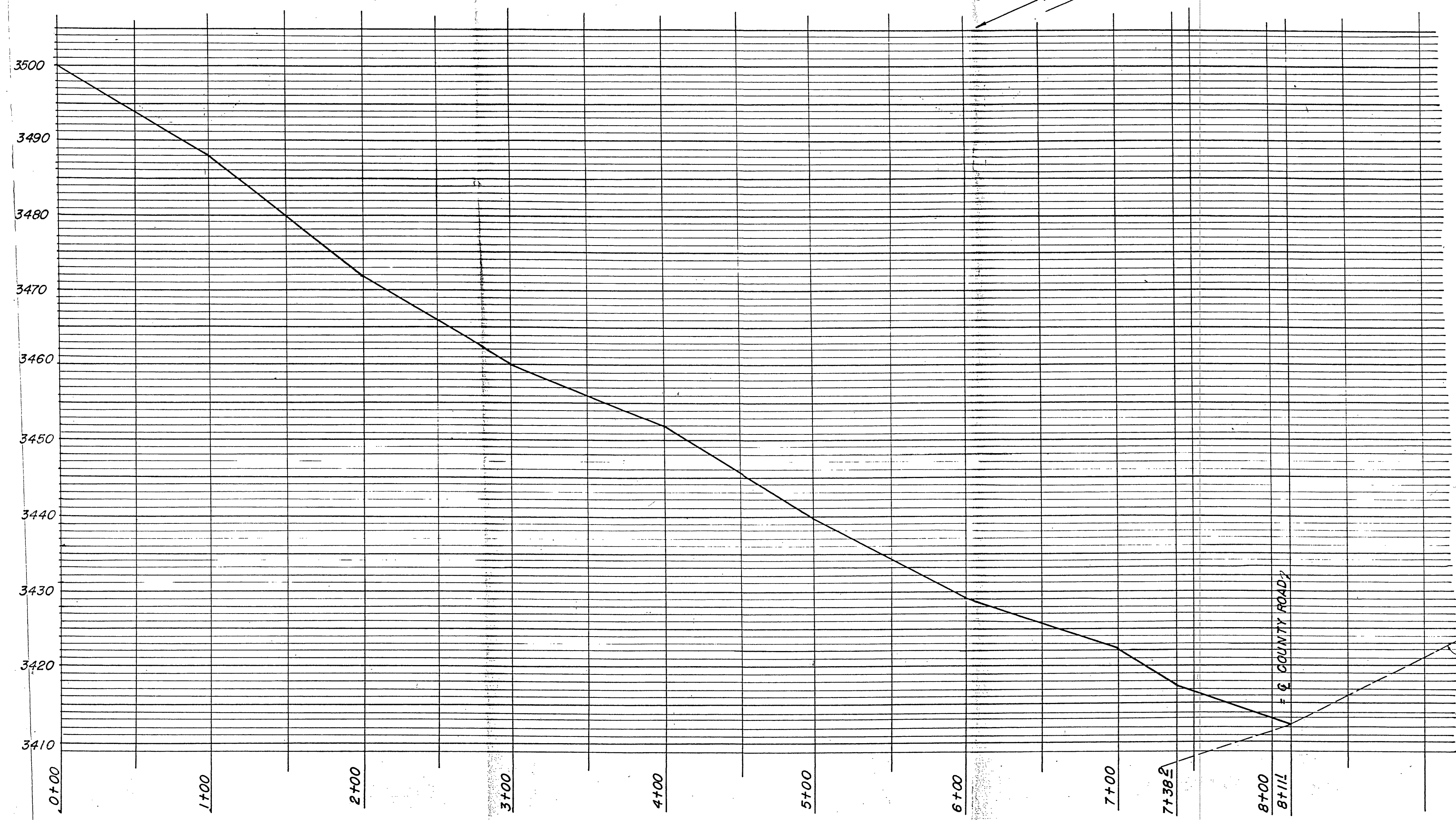
PROPOSED ROAD-PROFILE SCALE: 1" = 50' (Horiz.) 1" = 10' (Vert.)
